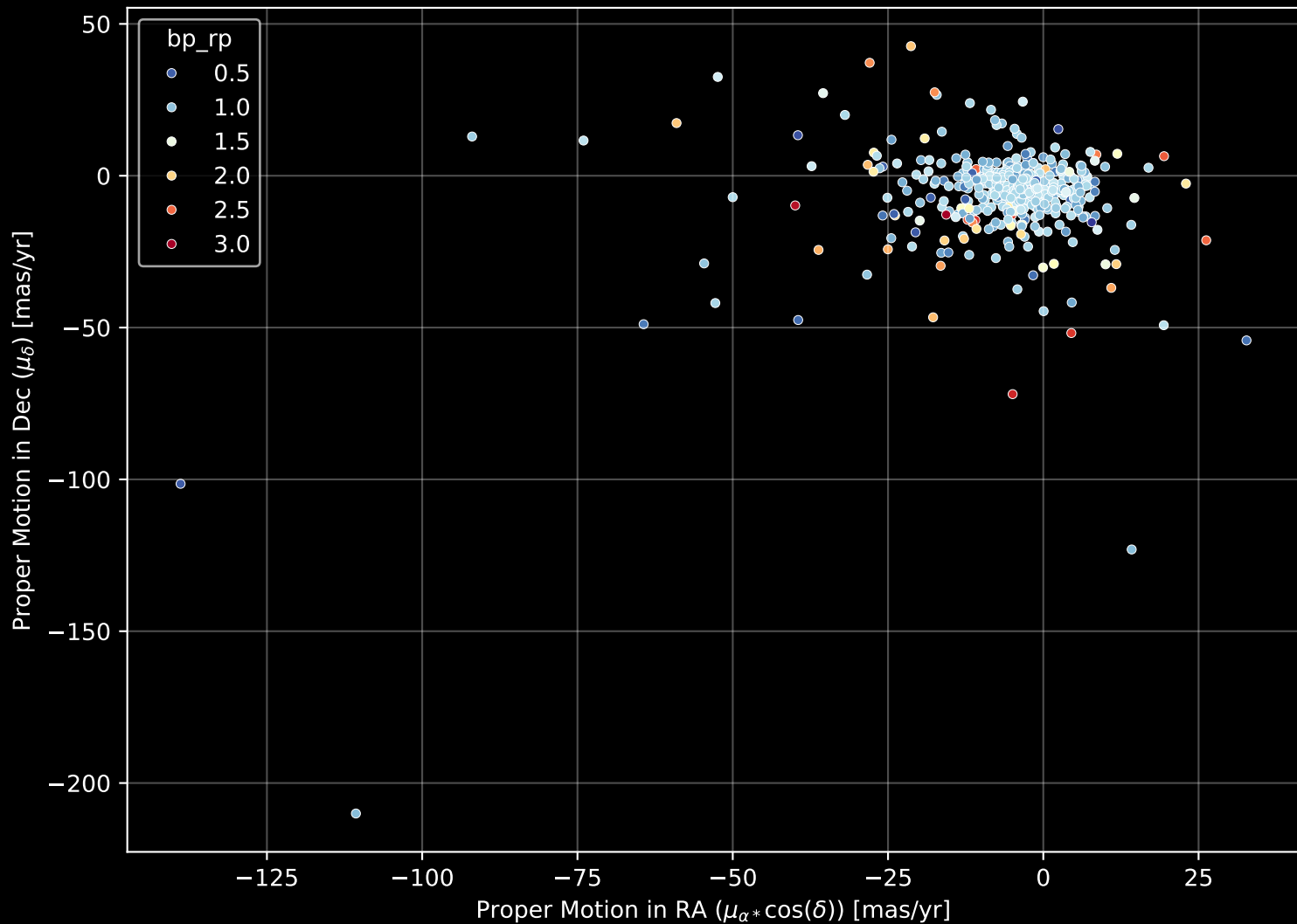
APOGEE DR17 Field: [PAL5-2] Proper Motion Diagram (n= 474)
