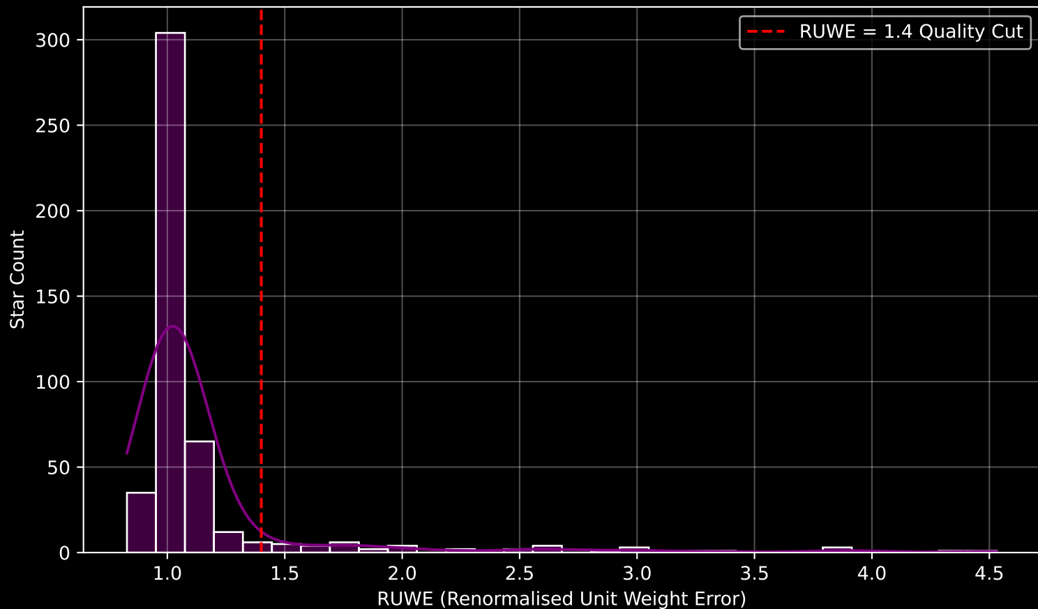
GAPOGEE DR17 Field [PAL5-2] RUWE Distribution (n= 463)
