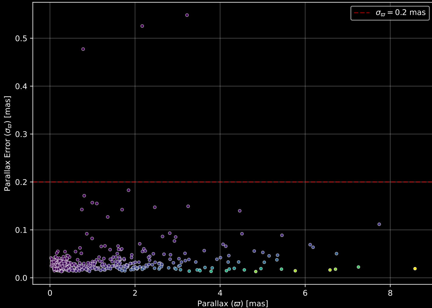
APOGEE DR17 Field: [PAL5-2] Parallax Quality (n= 474)
