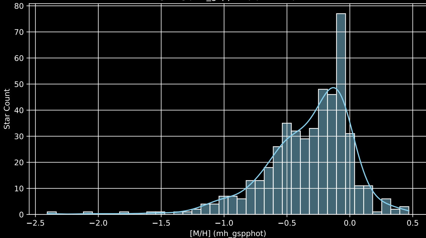
APOGEE DR17 Field: [PAL5-2 [M/H] (mh_gspphot) (n= 472)
