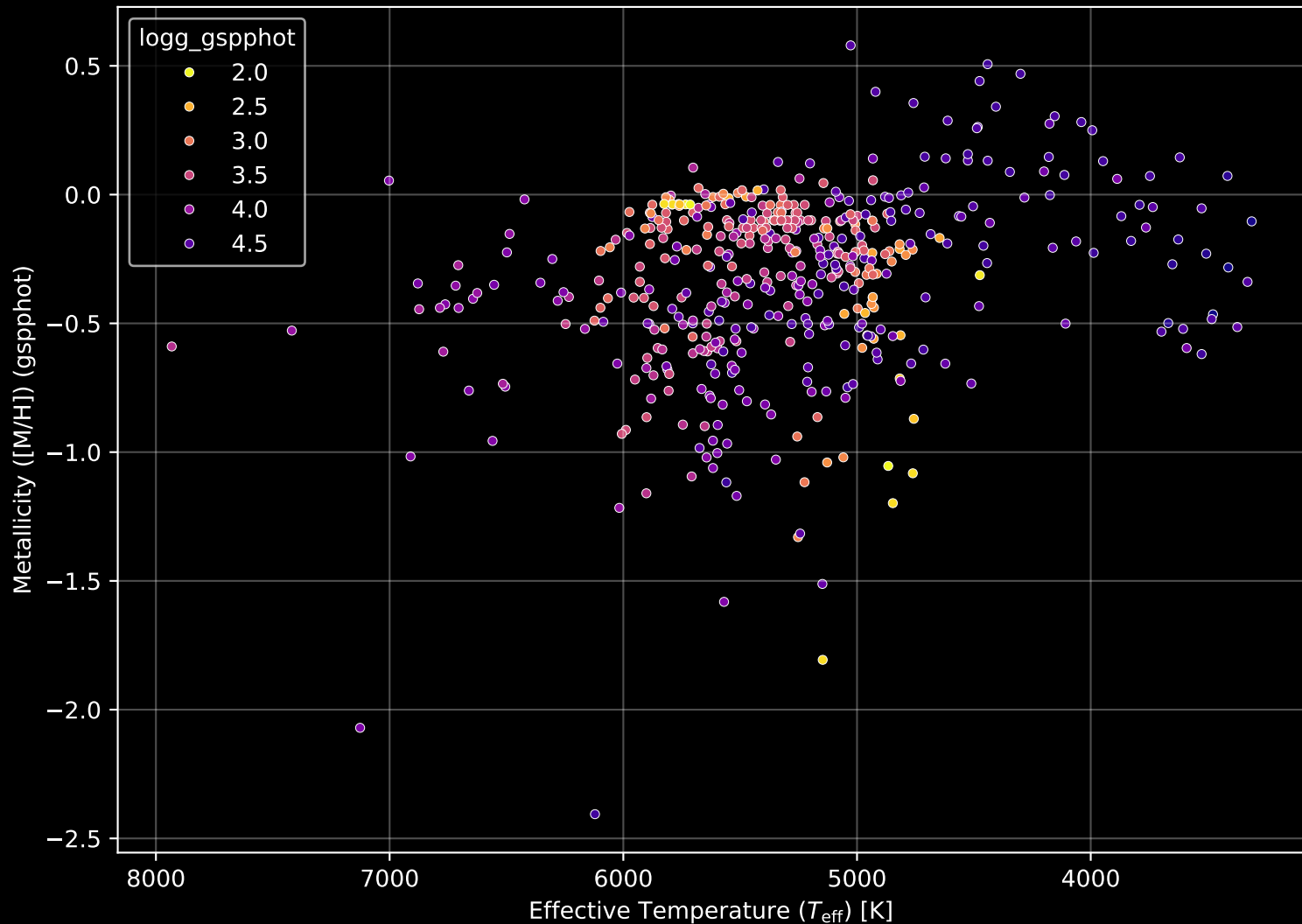
APOGEE DR17 Field: [PAL5-2] Stellar Population Parameters (n= 474)
