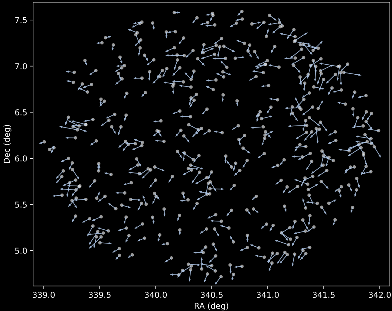
APOGEE DR17 Cluster 1 Proper Motion Vectors (n=391)
