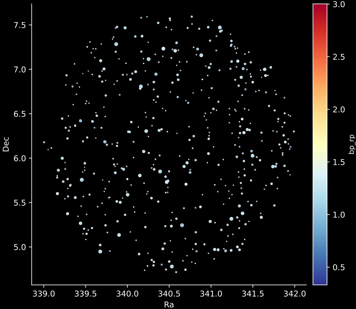
APOGEE DR17 Field: [PAL5-2] Stars: 474
